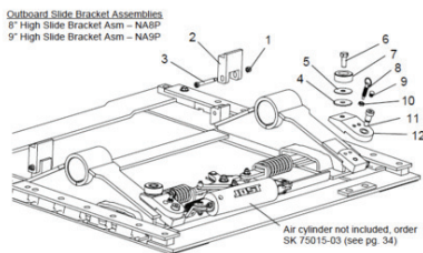
Slide Bracket Assembly 8" No-Tilt Convertible JOSNA8P
