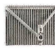
TA05-1203 Evaporator 7" x 10-3/8" x 2-5/8" OE# 3543-R0442001
